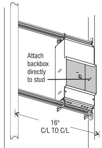
WALL MOUNT
