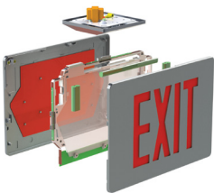
CONSTRUCTION VIEW
