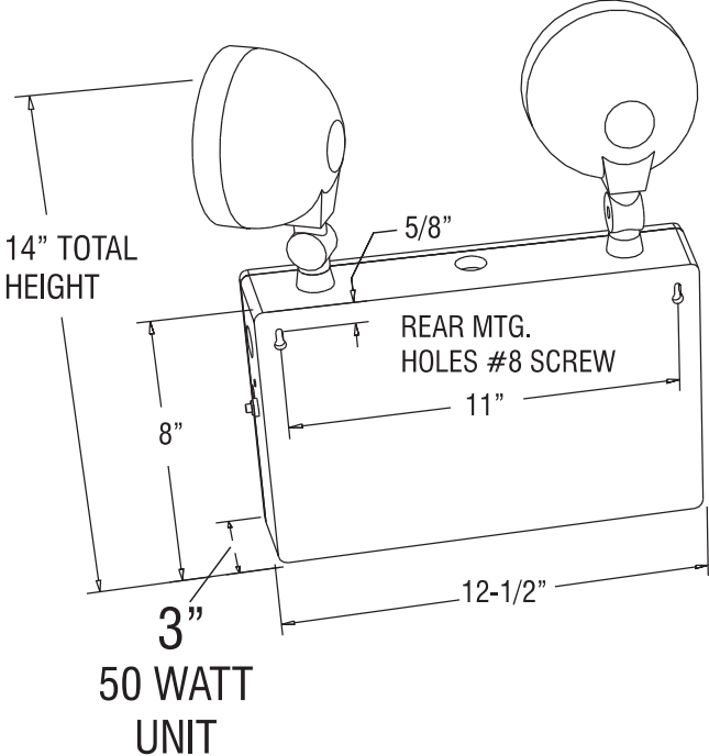
50 Watt and 100 Watt 6 or 12 Volt Unit Dimensions
