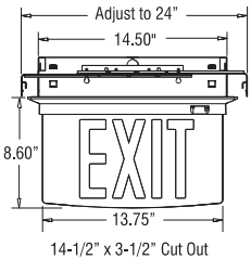
Recessed Ceiling Mount
