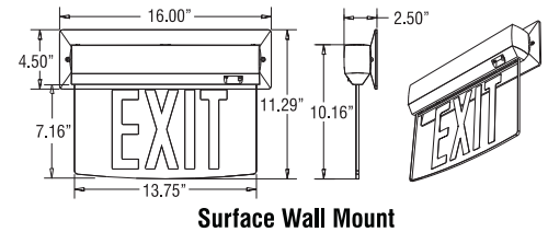
Surface Wall Mount
