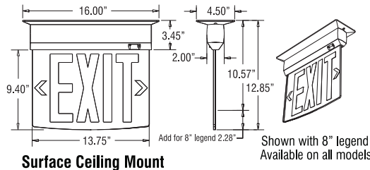
Surface Ceiling Mount
