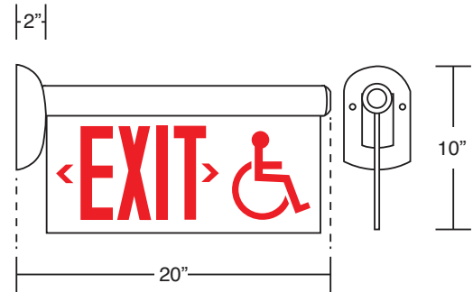
End Mount
