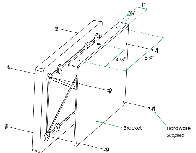
CEILING MOUNTING BRACKET For Single & Double Face
