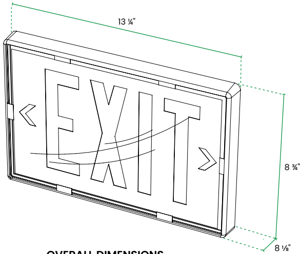
OVERALL DIMENSIONS
