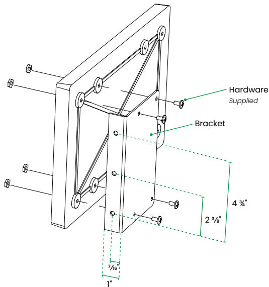
END MOUNTING BRACKET For Single & Double Face
