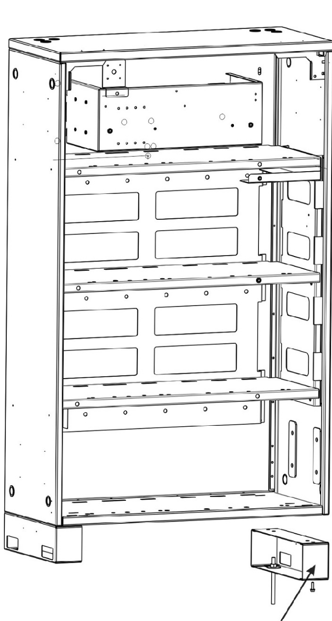
(2x) Floor Mounting Bracket
