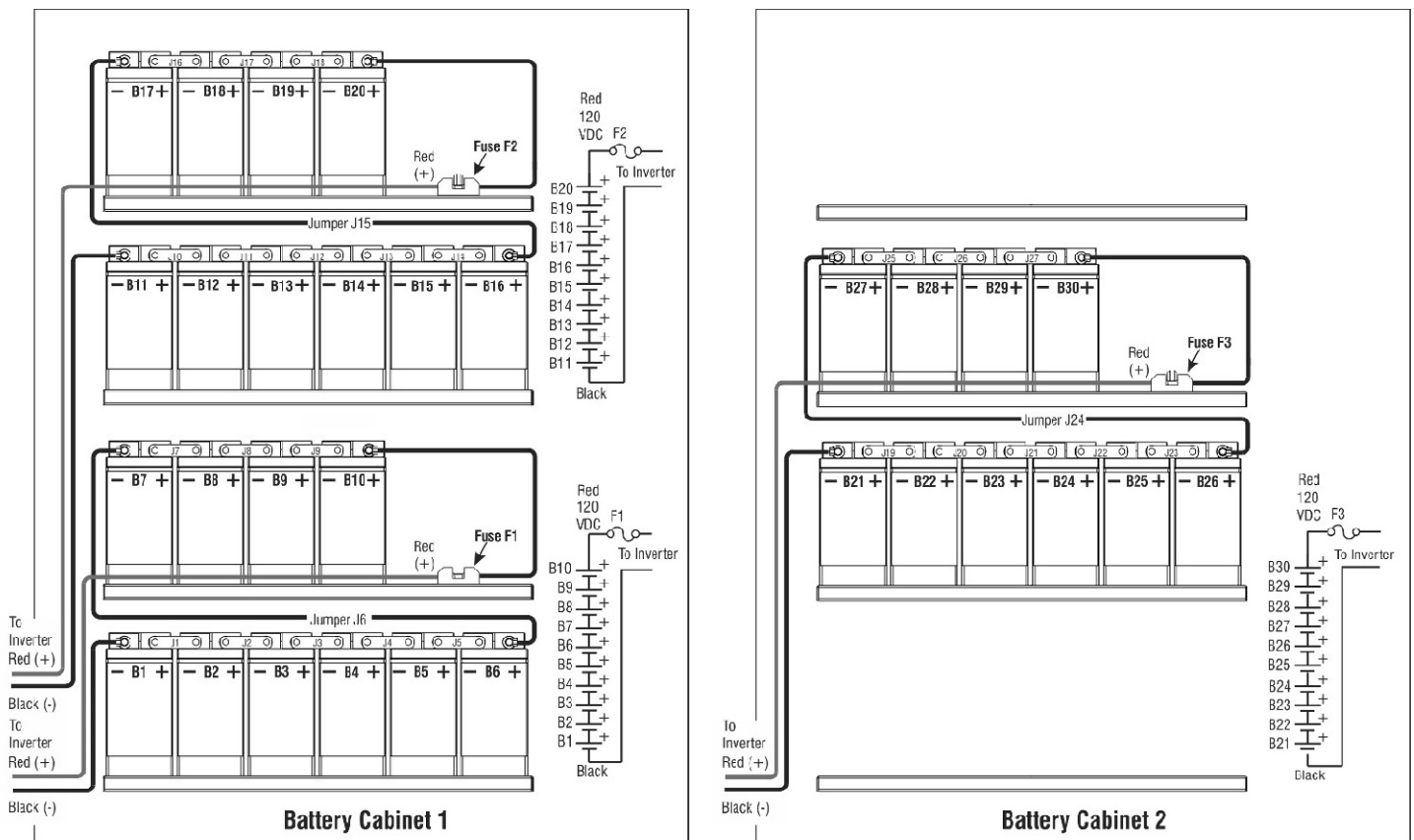
Three String Battery Connection - 120 VDC Systems
